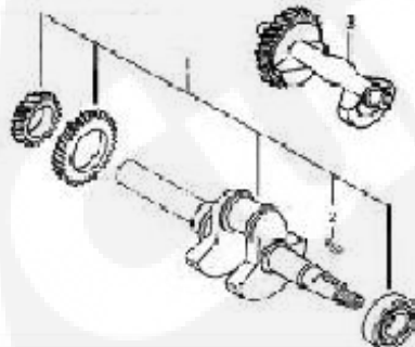
Crankshaft
