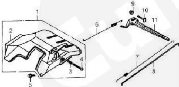
Speed Control
