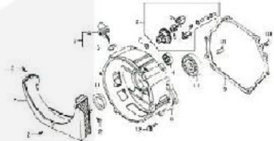
Starter
